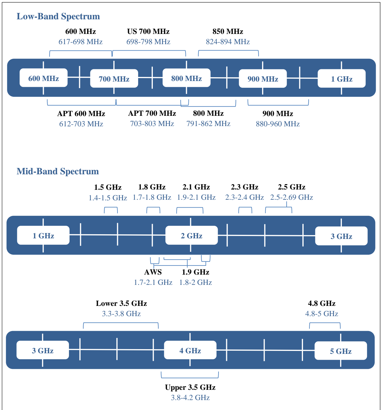
Figure 1: Cellular mobile frequency bands (low-band and mid-band spectrum)
