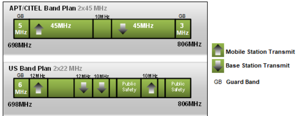
Figure 2: 700 MHz band plans
