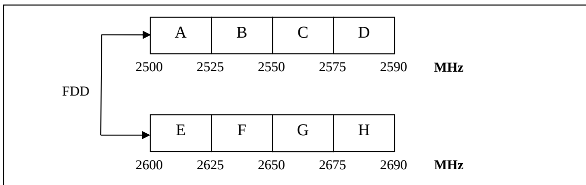
Figure 2: Frequency Assignment Plan for BWA Radiocommunication Systems in the 2.5 GHz Band
