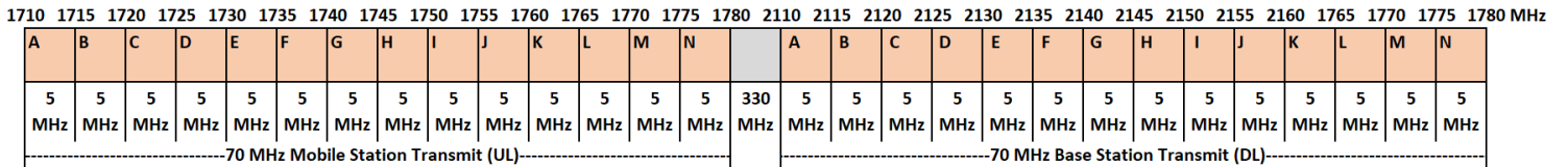
Figure 6. Frequency assignment plan for the AWS band
