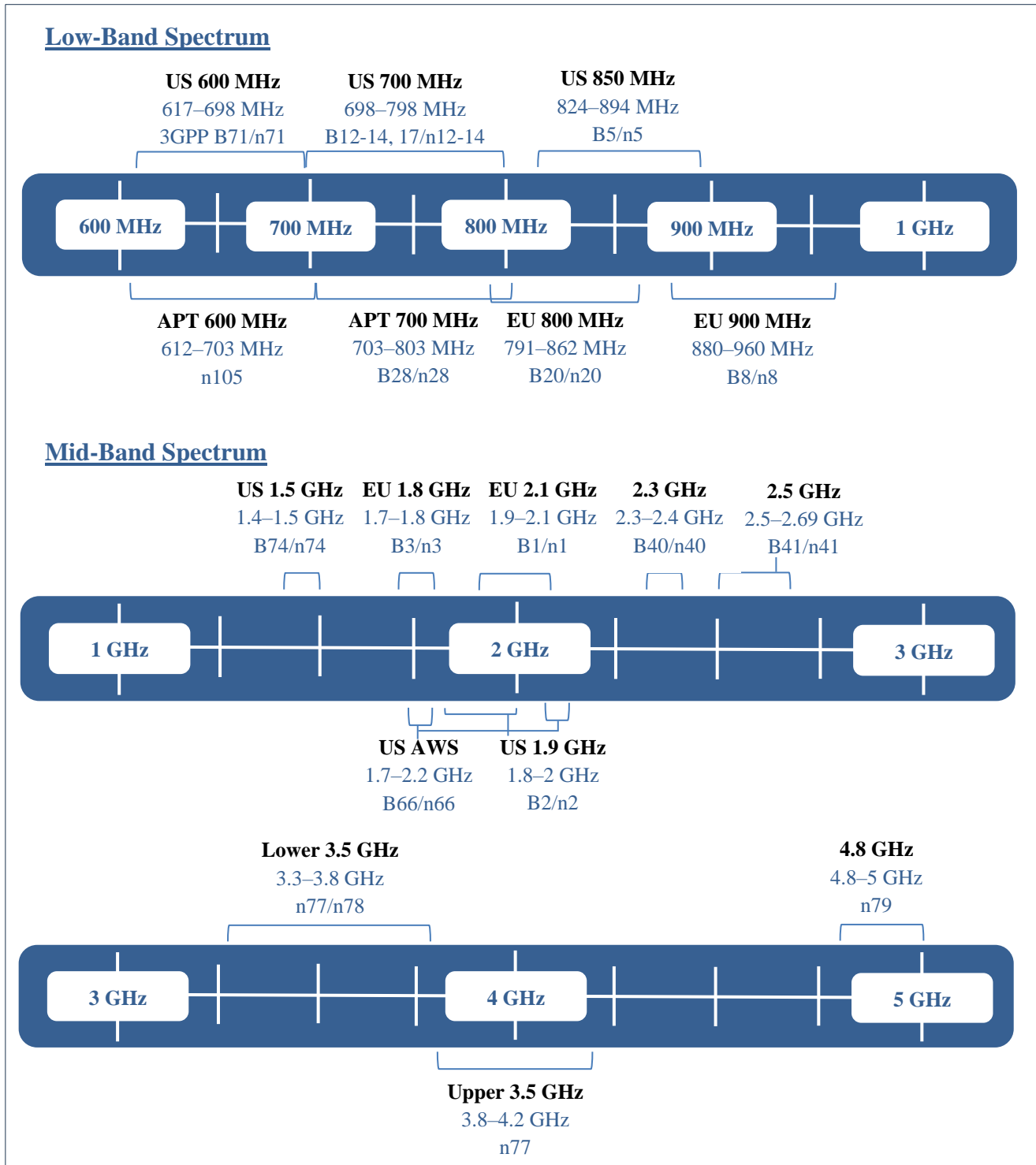
Figure 1. Cellular mobile frequency bands (low- and mid-band spectrum)
